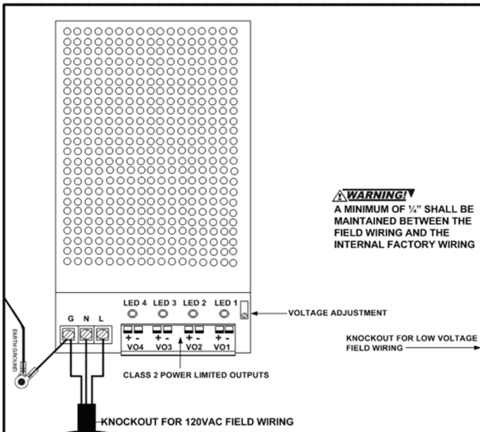
Output Terminal Block for circuits 1-4 and Voltage
